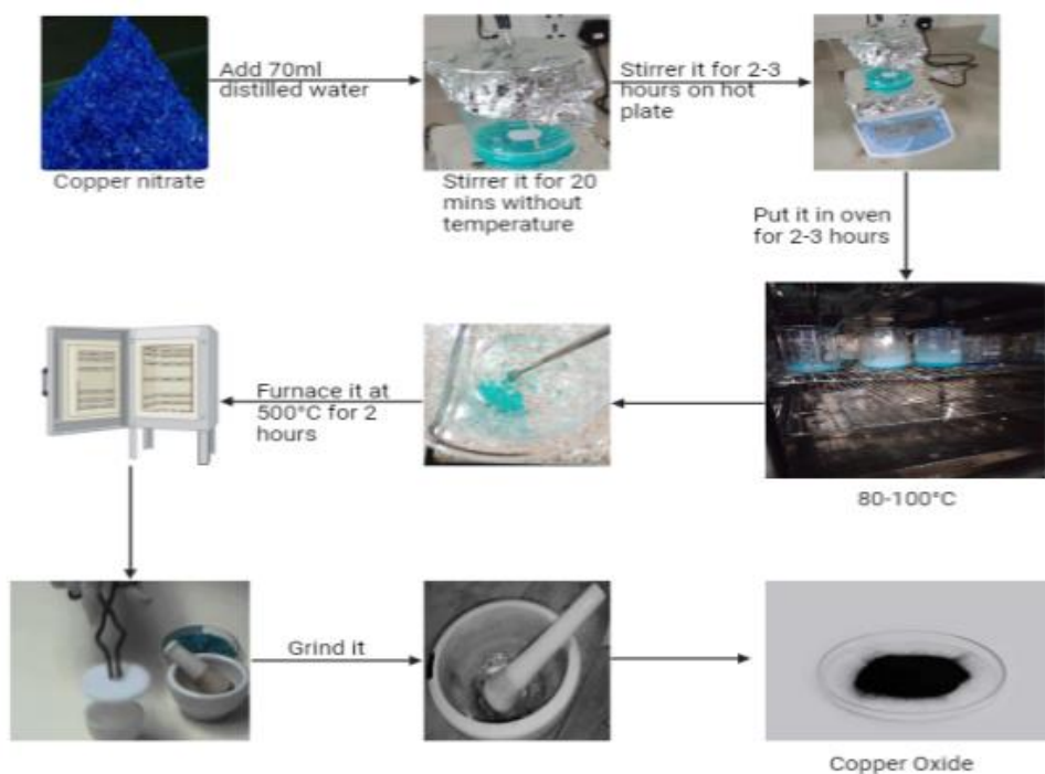
Figure 1: Systematic diagram of synthesis of copper oxide
