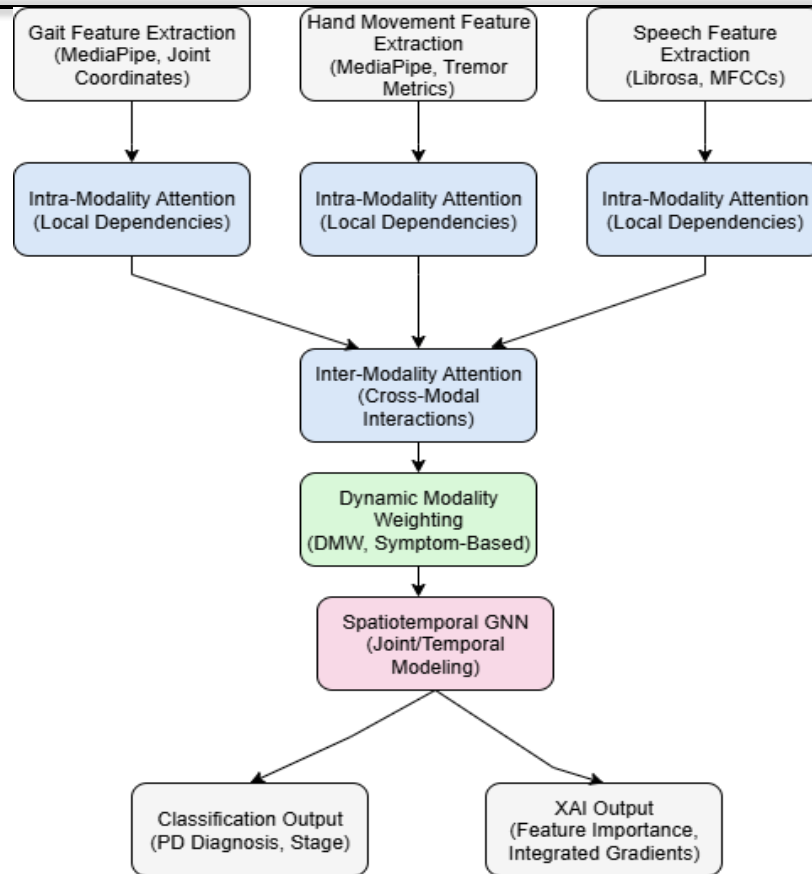
Figure 3: HAST-GNN-DMW Architecture
