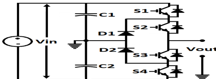
Fig. 3. Diode Clamped MLI with three level
