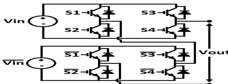
Fig. 4. Cascaded Multilevel Inverter with five levels.
