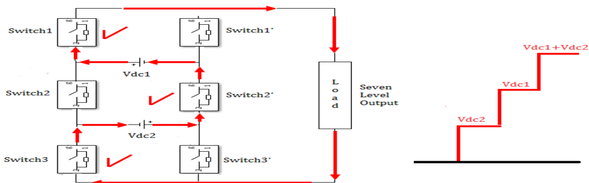
Fig. 9. Configuration & Current direction for Output level 3 of Switching
