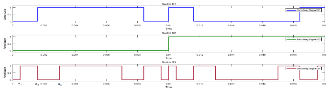
Fig. 16. S1, S2, & S3 switches in switching order.
