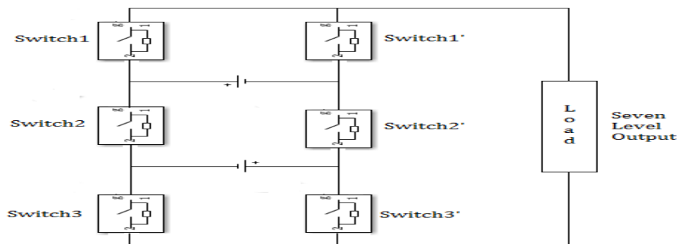
Fig. 5. The proposed Seven Level Inverter
