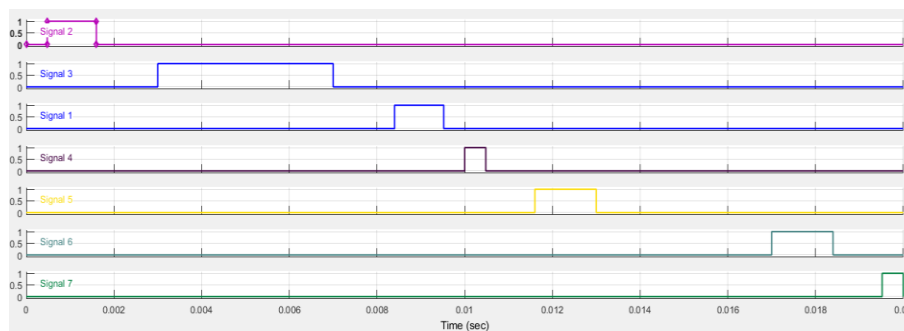
Fig. 14. Switching sequence 3 produced by Signal builder 2.
