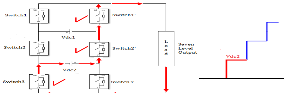
Fig. 7. Configuration & Current direction for Output level of Switching
