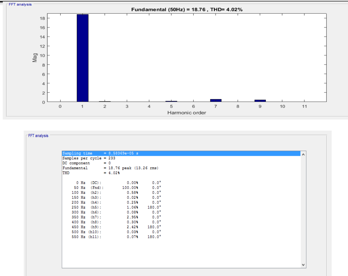
Fig. 17. Proposed Output voltage 7-level Inverter
