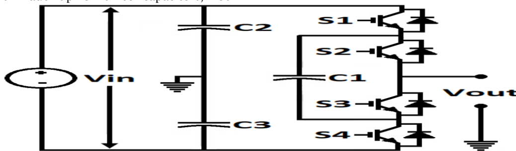
Fig. 2. Inverter of 3- Level Flying Capacitor having Multi Level
