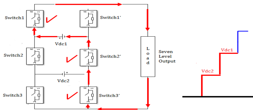
Fig. 8. Configuration & Current direction for Output level 2 of Switching
