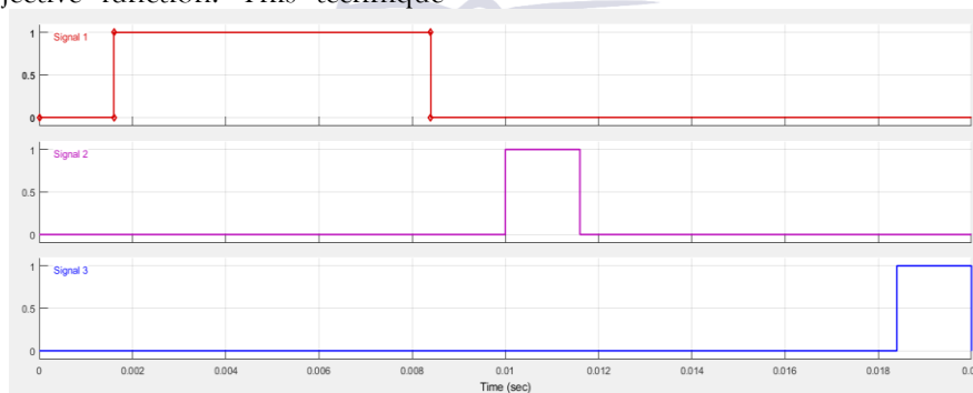
Fig. 13. Switching sequence 1 produced by Signal builder 1.
