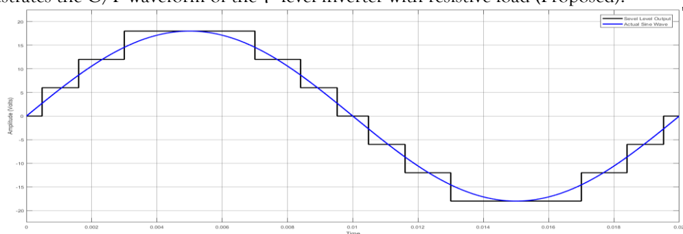
Fig. 15. 7-Level Inverter O/P waveform with resistive load (Proposed)
