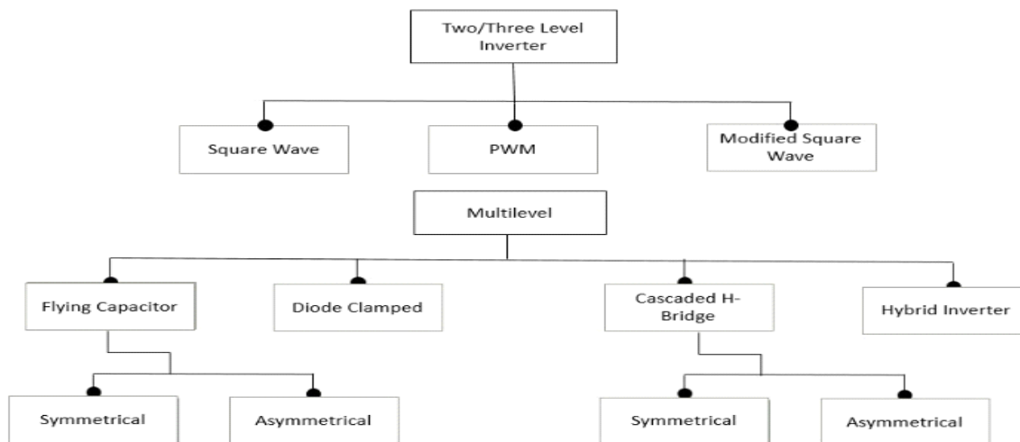
Fig. 1. Subtypes & Inverter types
