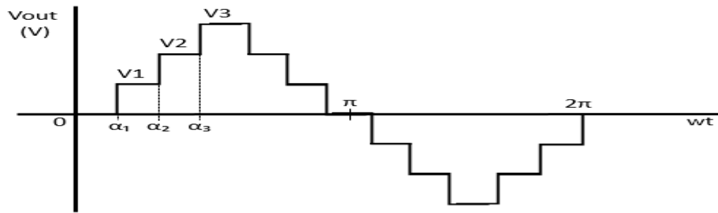
Fig. 11. Proposed 7-Level Inverter's output waveform complete cycle
