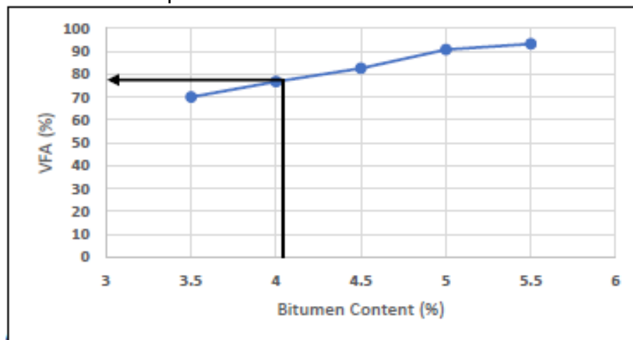
Figure 6: Bitumen Content vs. VFA
